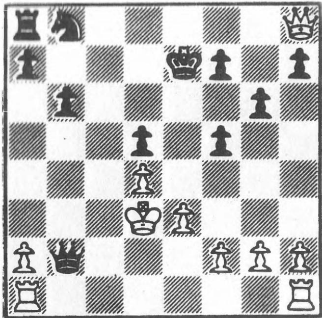
34 After 18 Kd3
